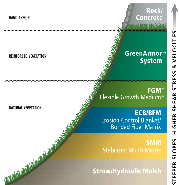
Figure 2: Performance Based on Slope, Shear Stress and Velocity
