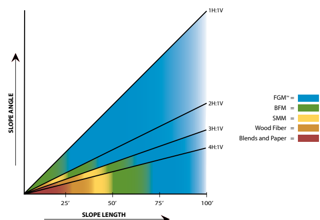
FIGURE 1: Hydraulically applied erosion control materials selection guideline
